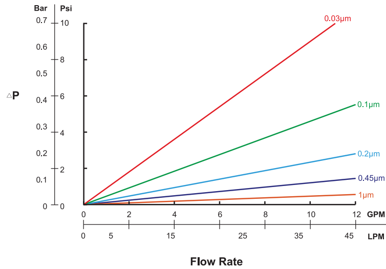
10" Polyethersulfone Membrane Pleated Filter Cartridge
